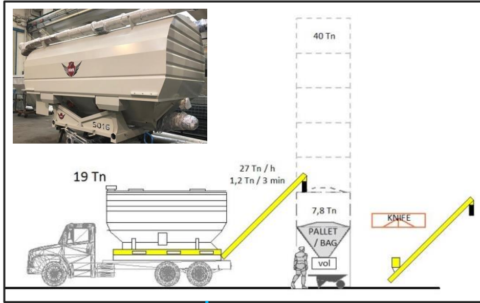
Delivery Bulk Truck
